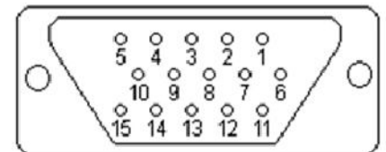
VGA CONNECTOR FRONT VIEW
