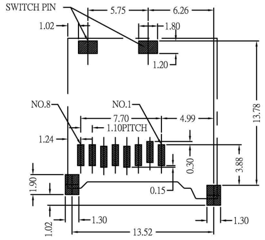
PCB LARYUOT(GENERAL TOLERANCE±0.05mm)
